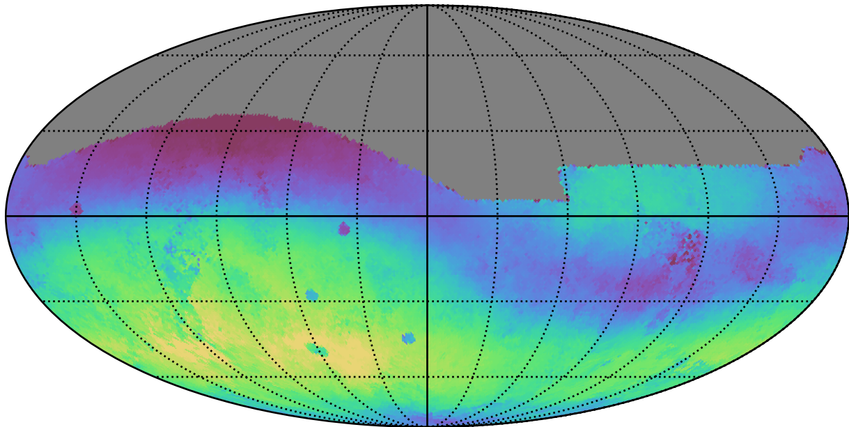
extra_ss_neo4_v3.4_10yrs All sky g band: Median skyBrightness
