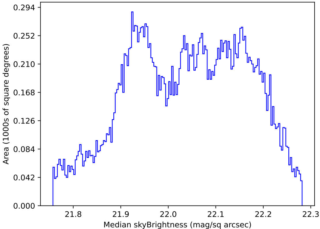
extra_ss_neo4_v3.4_10yrs All sky g band: Median skyBrightness
