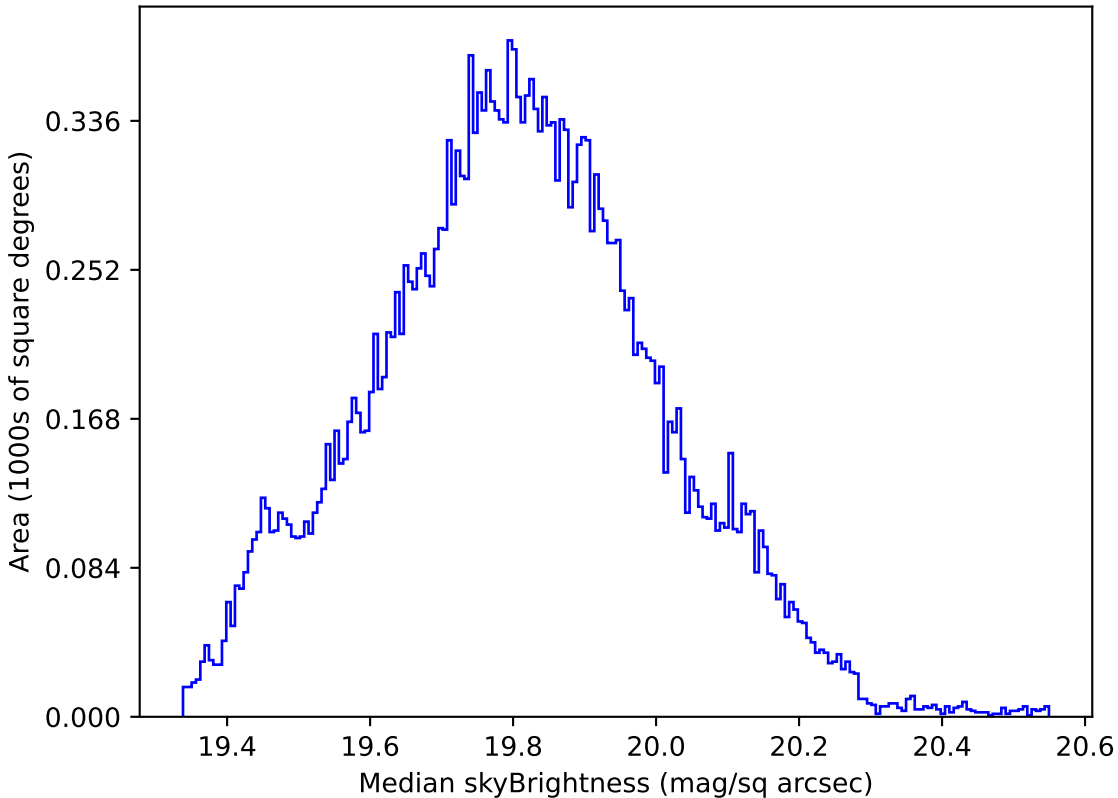
extra_ss_neo4_v3.4_10yrs All sky all bands: Median skyBrightness
