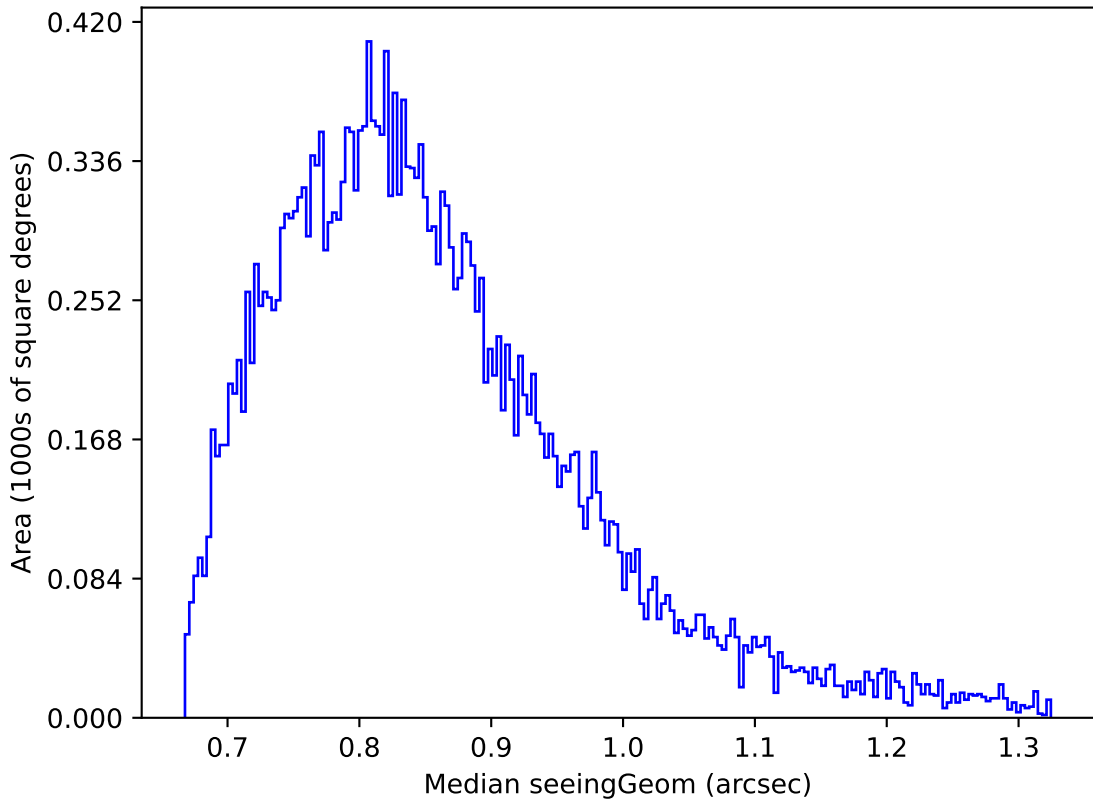
extra_ss_neo4_v3.4_10yrs Yr 1 z band: Median seeingGeom
