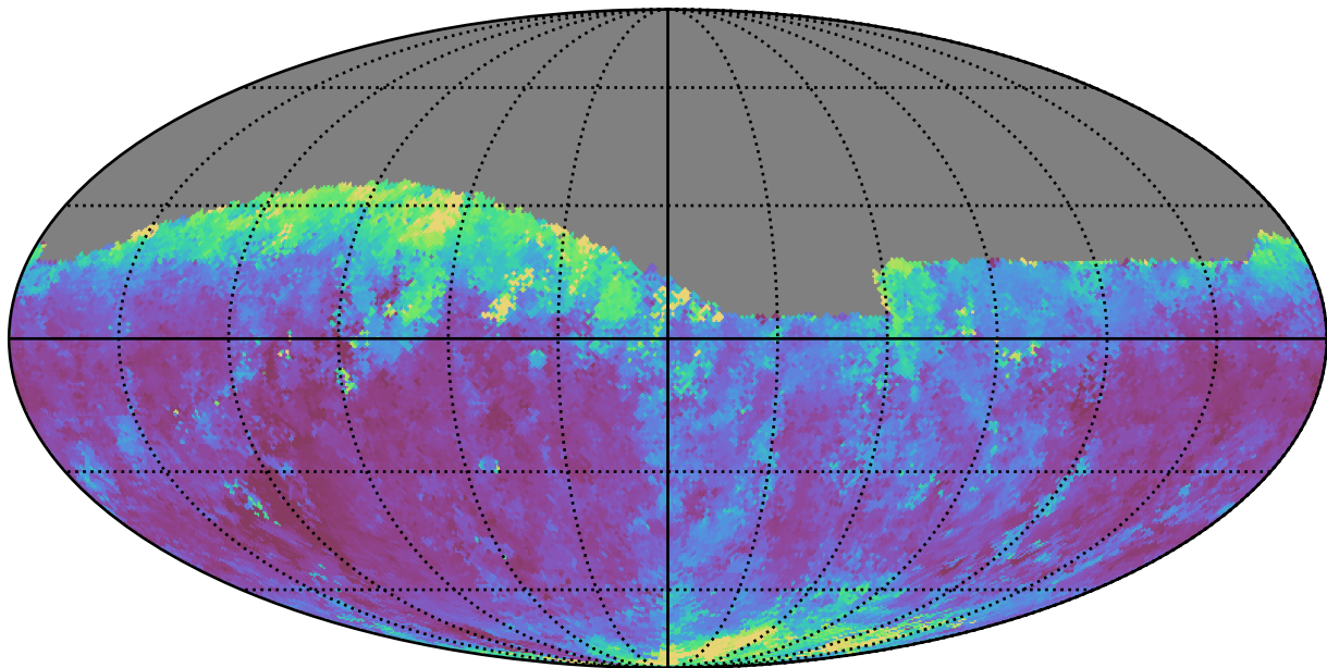
extra_ss_neo4_v3.4_10yrs Yr 1 r band: Median seeingGeom
