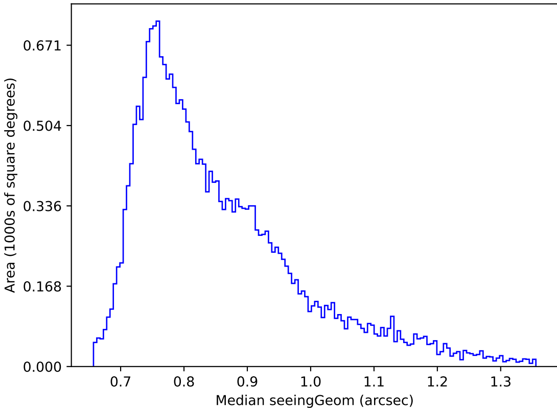
extra_ss_neo4_v3.4_10yrs Yr 1 r band: Median seeingGeom
