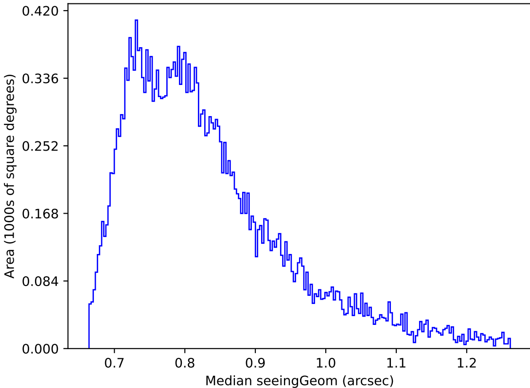
extra_ss_neo4_v3.4_10yrs Yr 1 i band: Median seeingGeom
