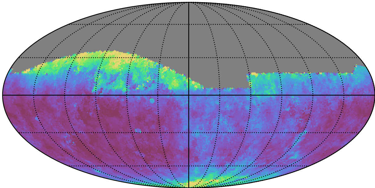
extra_ss_neo4_v3.4_10yrs Yr 1 all bands: Median seeingGeom
