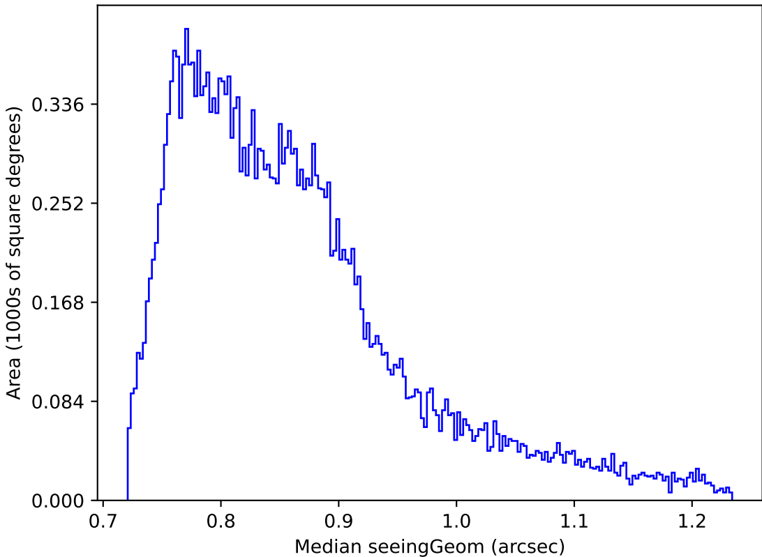
extra_ss_neo4_v3.4_10yrs Yr 1 all bands: Median seeingGeom
