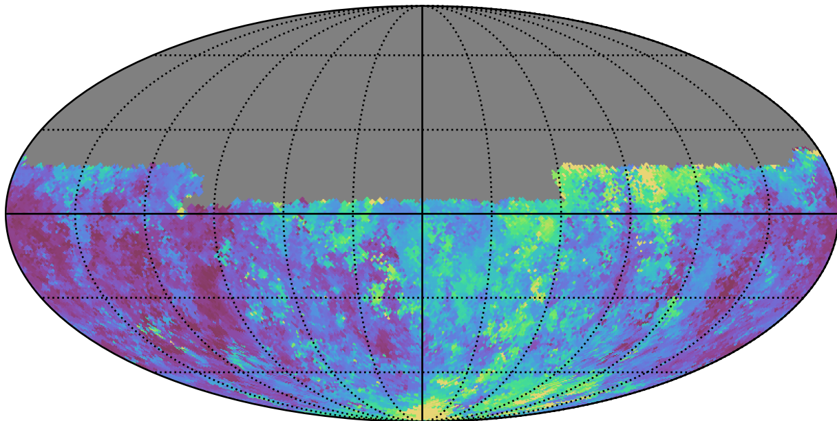
extra_ss_neo4_v3.4_10yrs Yr 1 u band: Median seeingEff
