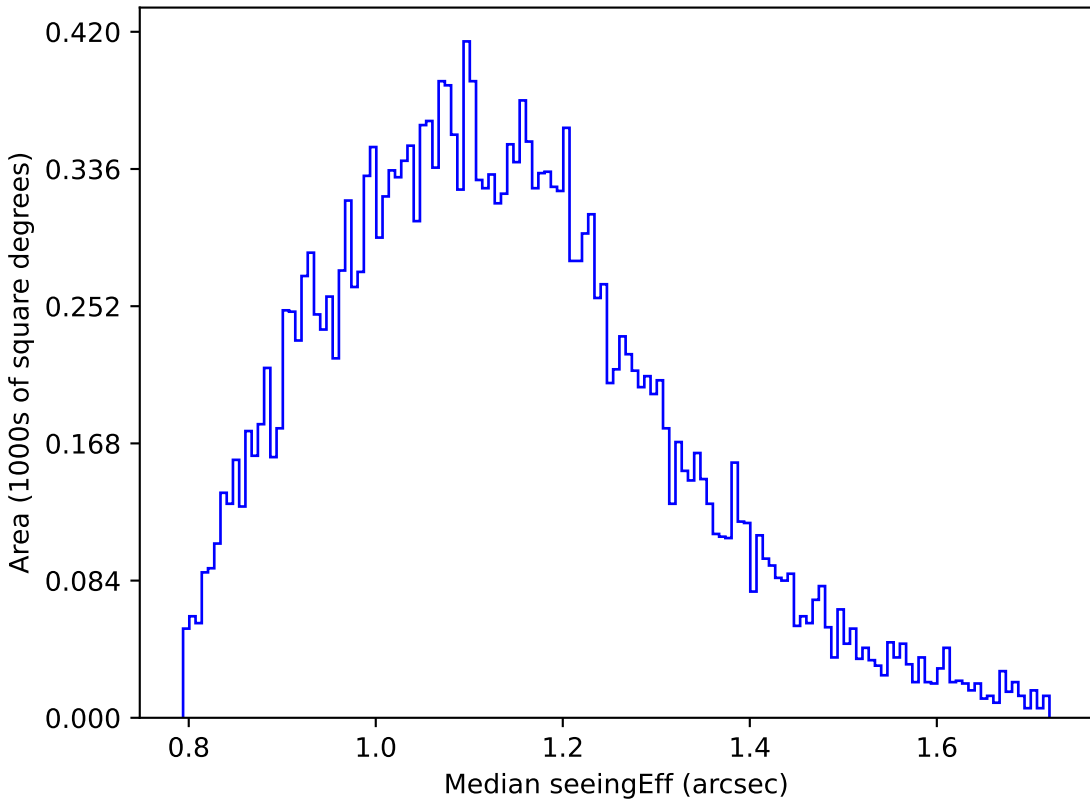
extra_ss_neo4_v3.4_10yrs Yr 1 u band: Median seeingEff
