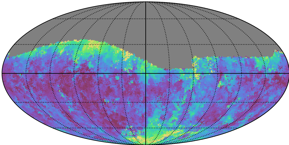
extra_ss_neo4_v3.4_10yrs Yr 1 g band: Median seeingEff
