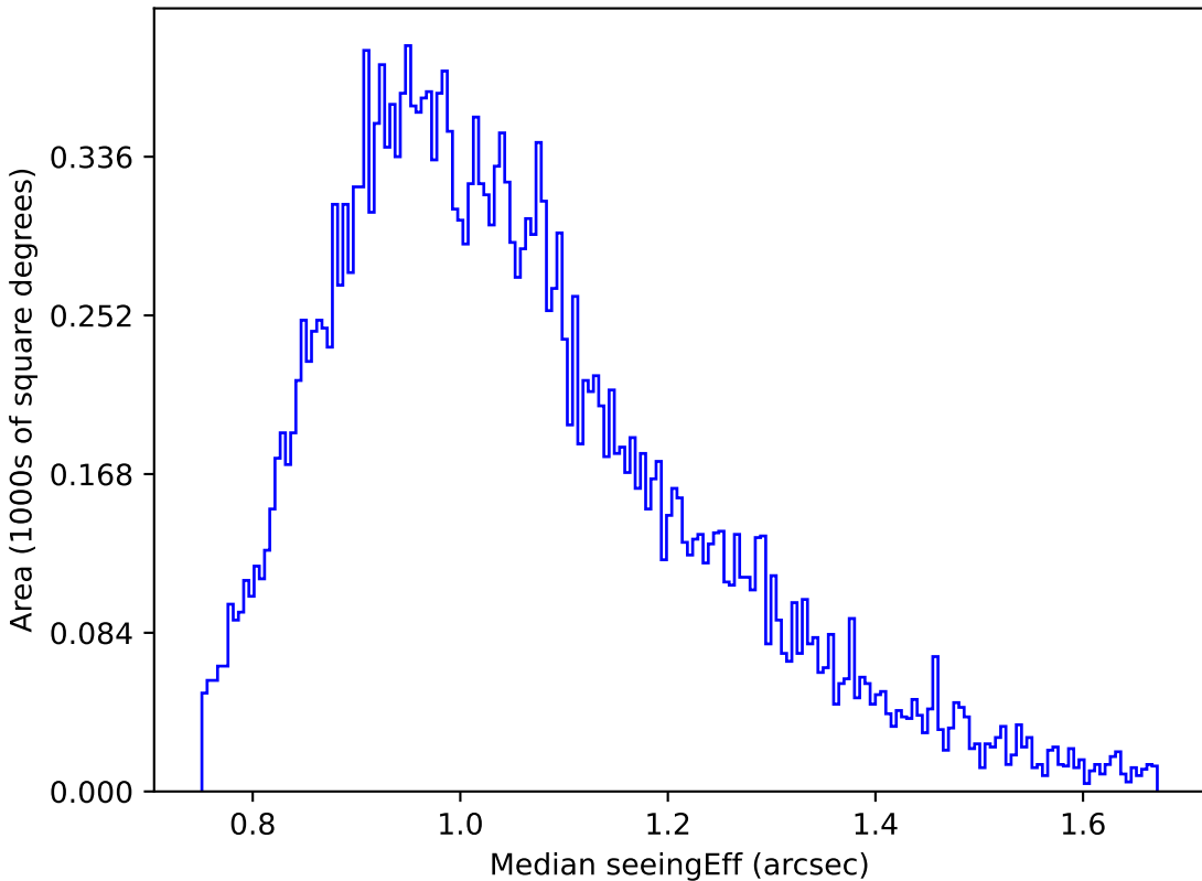
extra_ss_neo4_v3.4_10yrs Yr 1 g band: Median seeingEff
