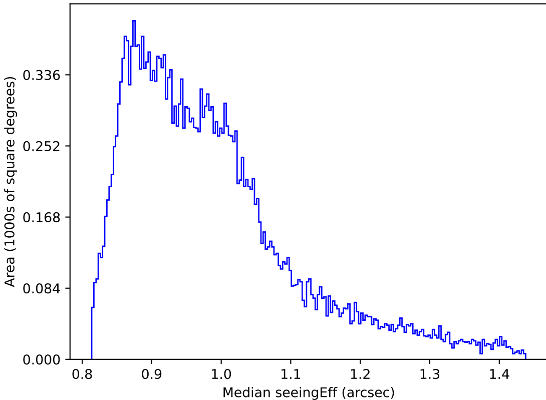
extra_ss_neo4_v3.4_10yrs Yr 1 all bands: Median seeingEff
