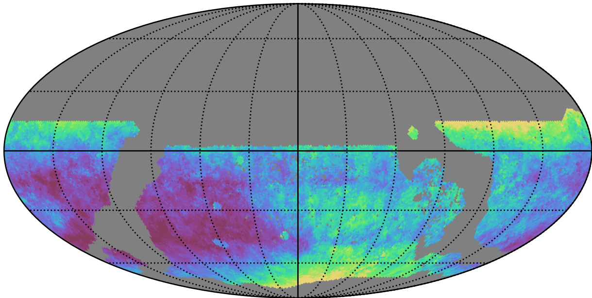
extra_ss_neo4_v3.4_10yrs WFD z band: Median seeingEff
