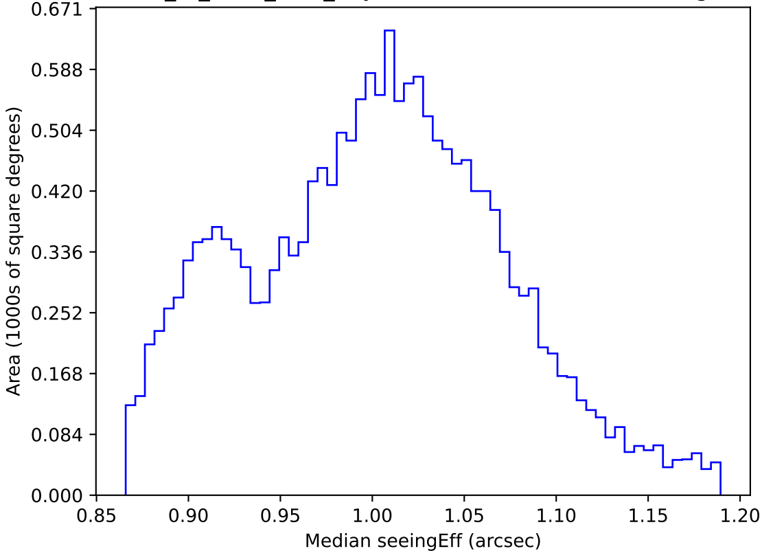
extra_ss_neo4_v3.4_10yrs WFD z band: Median seeingEff
