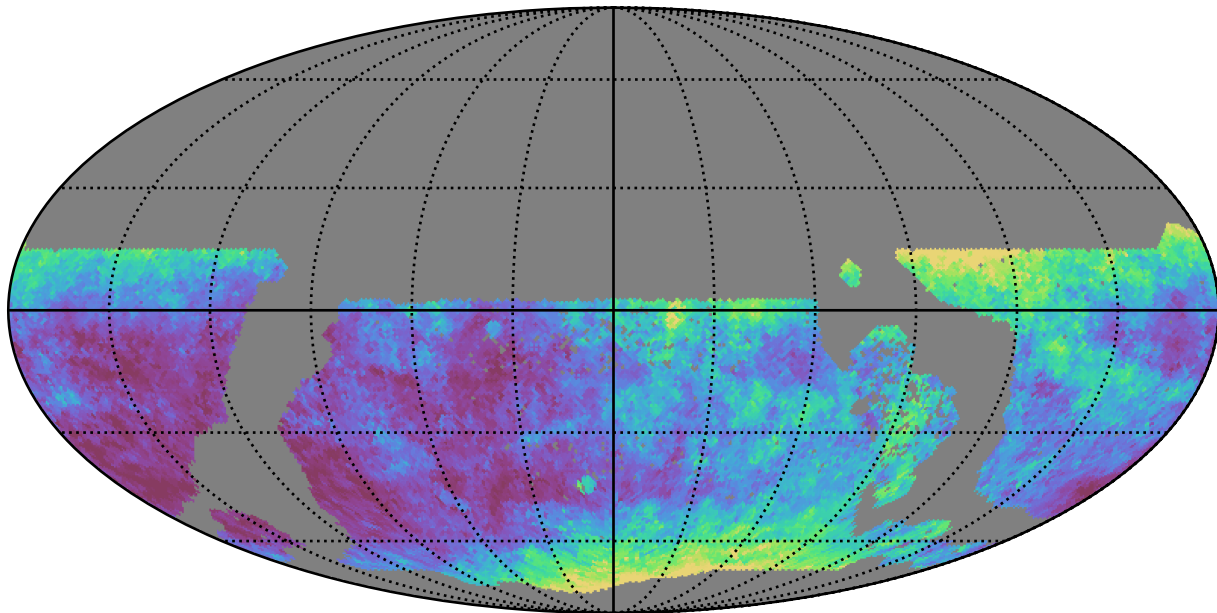
extra_ss_neo4_v3.4_10yrs WFD y band: Median seeingEff
