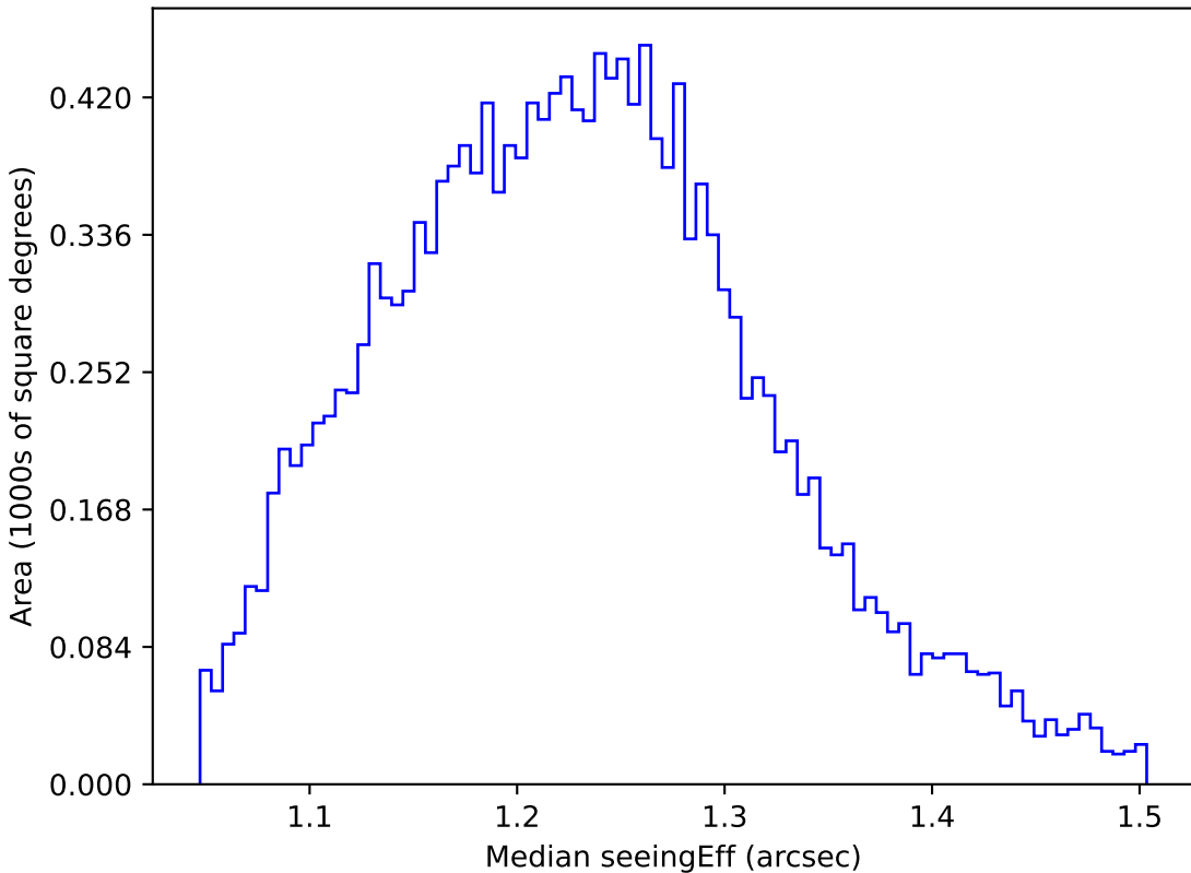
extra_ss_neo4_v3.4_10yrs WFD u band: Median seeingEff
