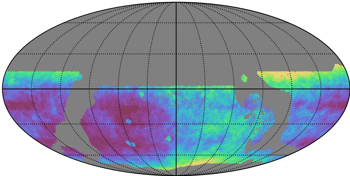
extra_ss_neo4_v3.4_10yrs WFD r band: Median seeingEff
