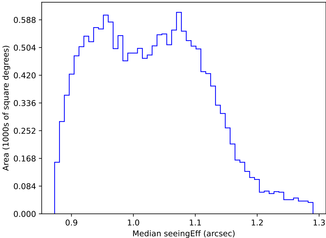
extra_ss_neo4_v3.4_10yrs WFD r band: Median seeingEff
