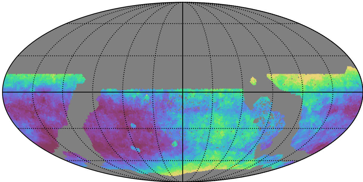
extra_ss_neo4_v3.4_10yrs WFD i band: Median seeingEff
