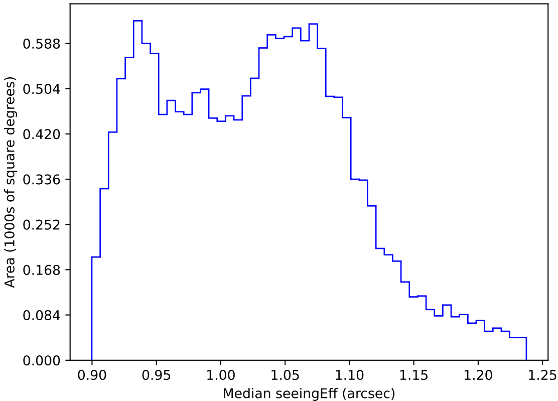
extra_ss_neo4_v3.4_10yrs WFD all bands: Median seeingEff
