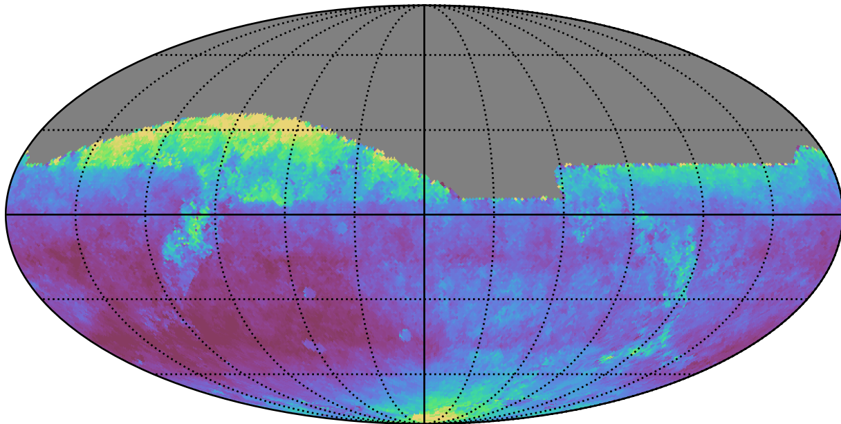
extra_ss_neo4_v3.4_10yrs All sky z band: Median seeingEff
