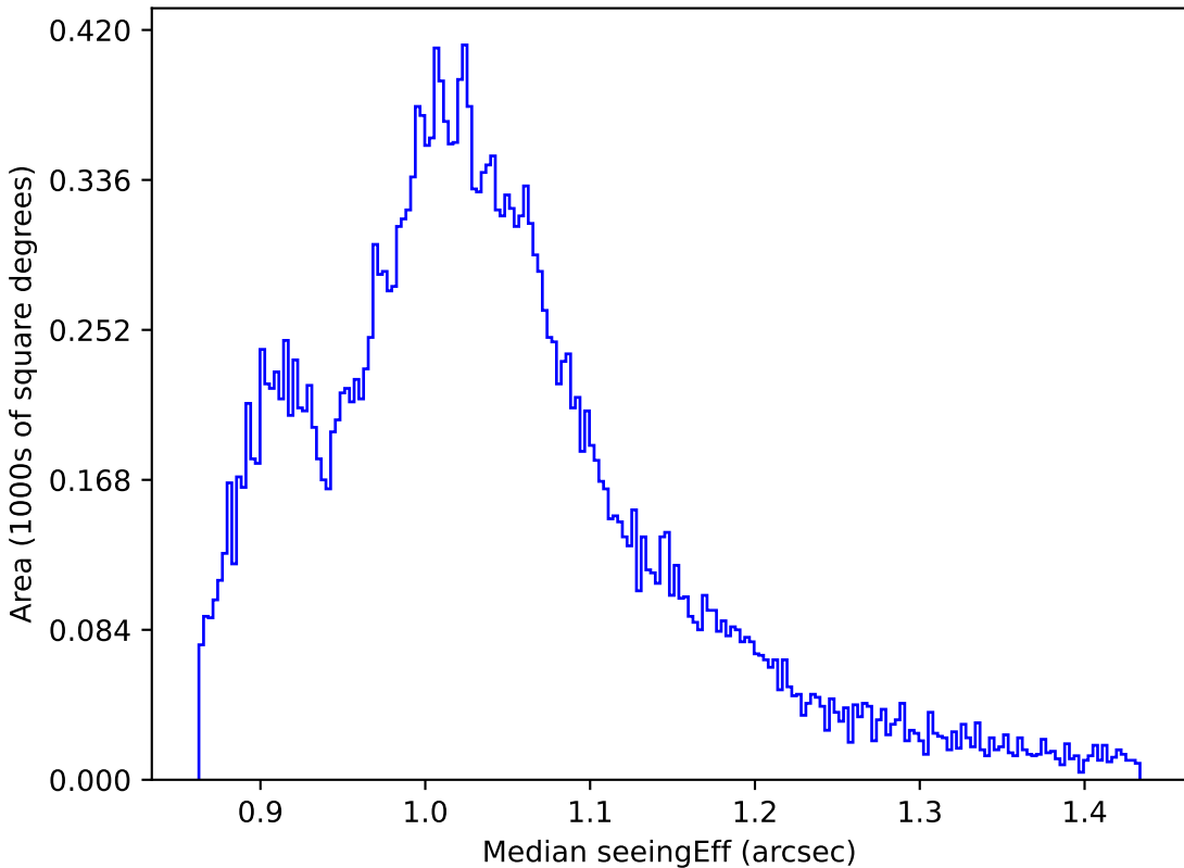
extra_ss_neo4_v3.4_10yrs All sky z band: Median seeingEff
