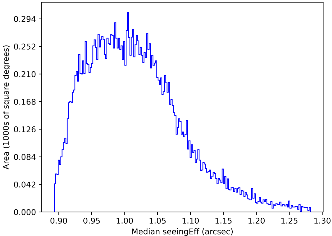
extra_ss_neo4_v3.4_10yrs All sky y band: Median seeingEff
