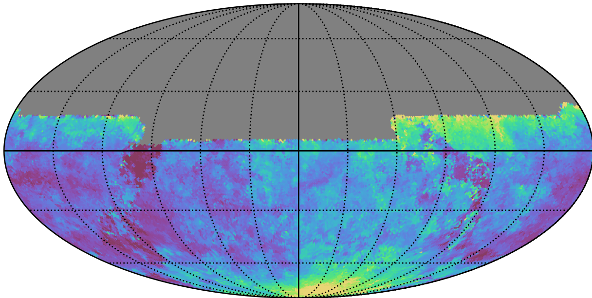
extra_ss_neo4_v3.4_10yrs All sky u band: Median seeingEff
