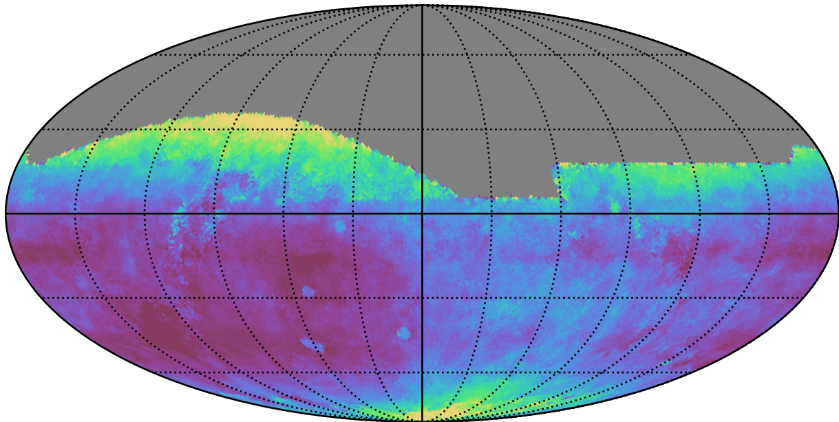
extra_ss_neo4_v3.4_10yrs All sky r band: Median seeingEff
