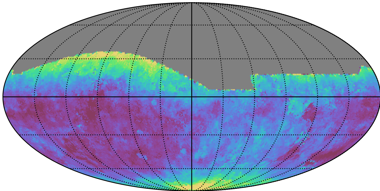
extra_ss_neo4_v3.4_10yrs All sky g band: Median seeingEff
