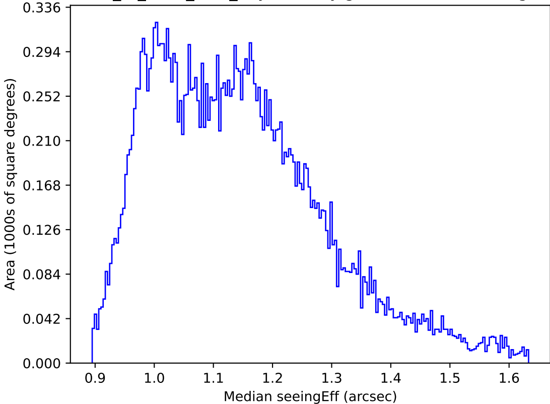
extra_ss_neo4_v3.4_10yrs All sky g band: Median seeingEff
