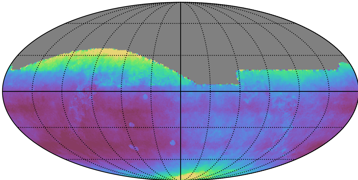
extra_ss_neo4_v3.4_10yrs All sky all bands: Median seeingEff
