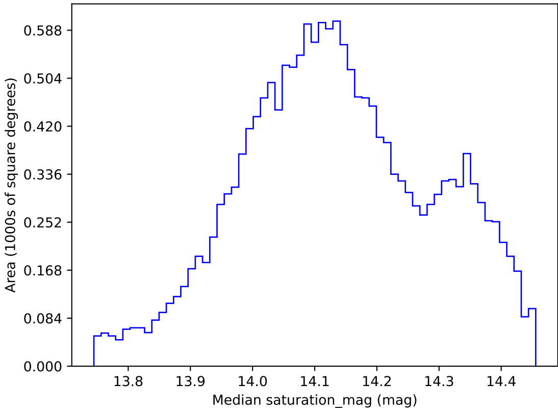
extra_ss_neo4_v3.4_10yrs WFD z band: Median saturation_mag
