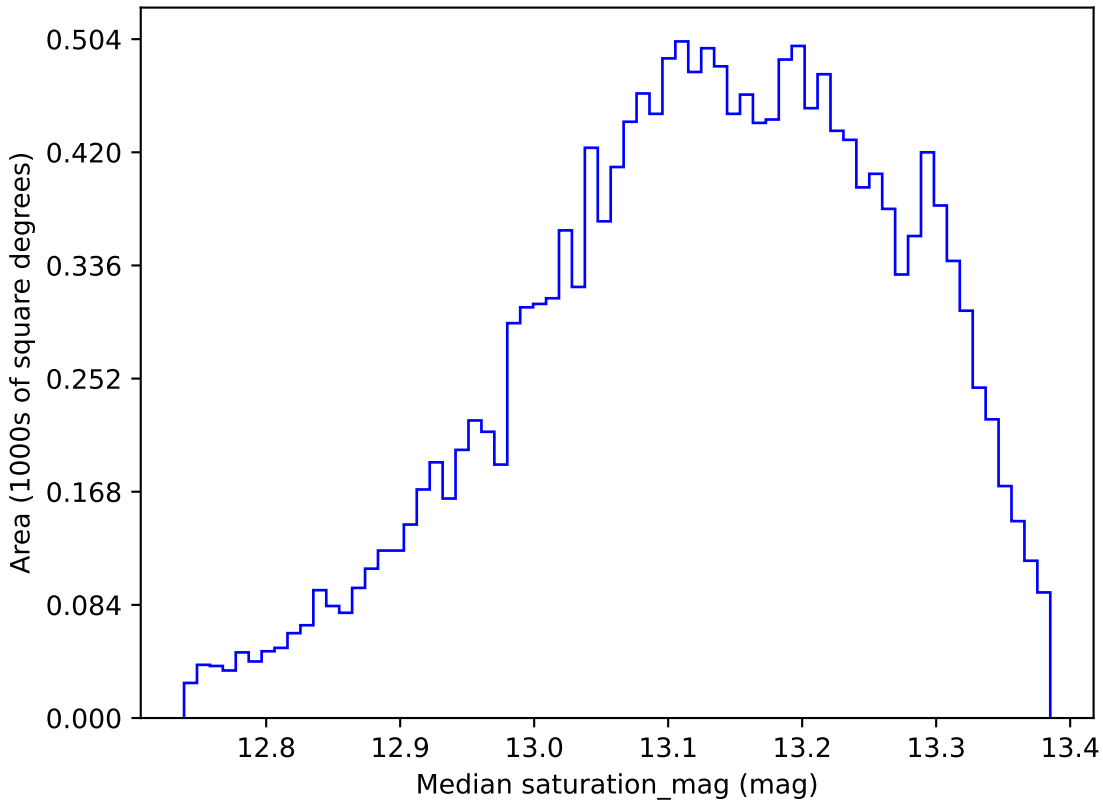
extra_ss_neo4_v3.4_10yrs WFD y band: Median saturation_mag
