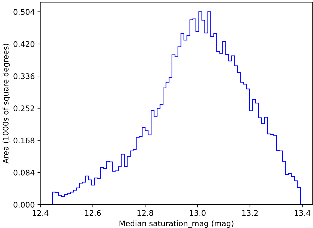
extra_ss_neo4_v3.4_10yrs WFD u band: Median saturation_mag
