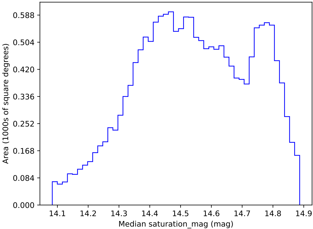
extra_ss_neo4_v3.4_10yrs WFD i band: Median saturation_mag
