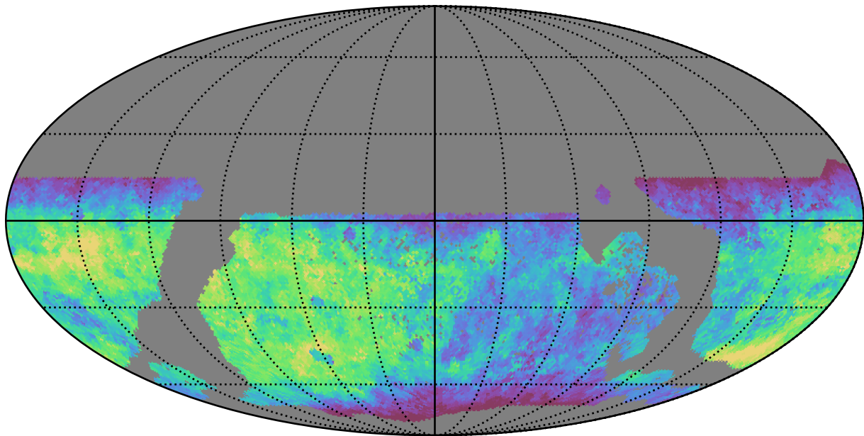
extra_ss_neo4_v3.4_10yrs WFD g band: Median saturation_mag
