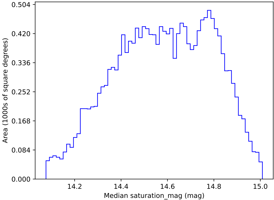
extra_ss_neo4_v3.4_10yrs WFD g band: Median saturation_mag
