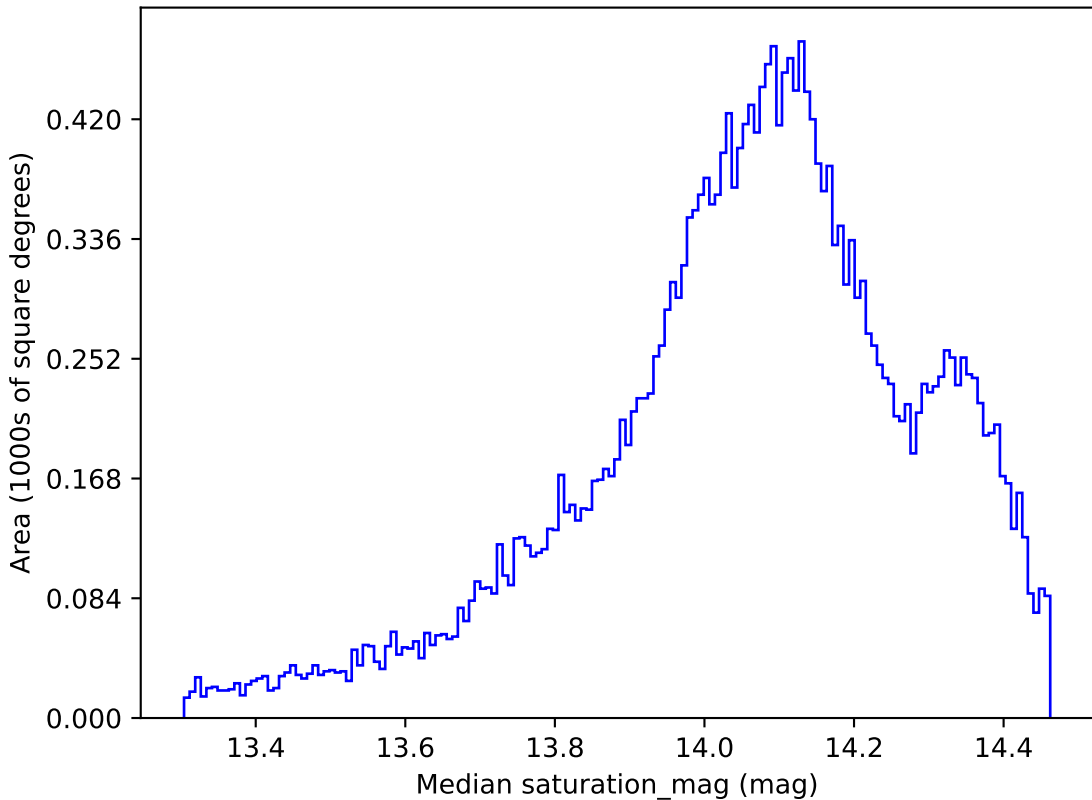
extra_ss_neo4_v3.4_10yrs All sky z band: Median saturation_mag
