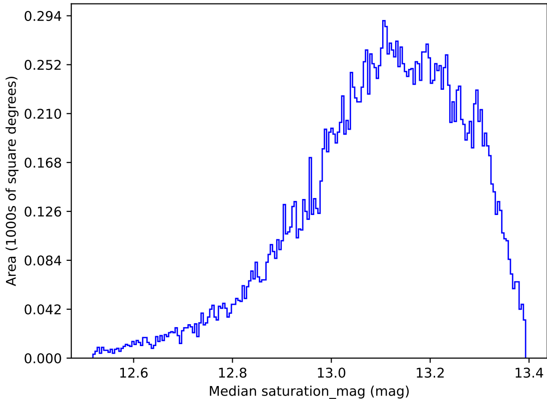
extra_ss_neo4_v3.4_10yrs All sky y band: Median saturation_mag
