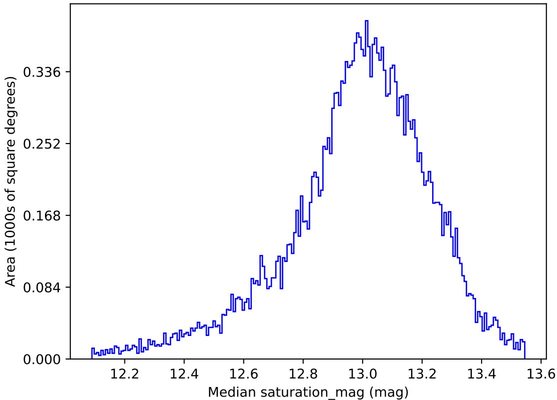
extra_ss_neo4_v3.4_10yrs All sky u band: Median saturation_mag
