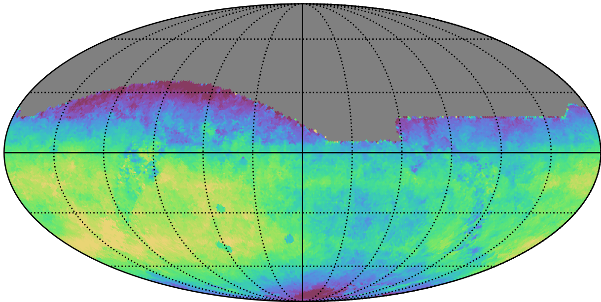
extra_ss_neo4_v3.4_10yrs All sky i band: Median saturation_mag
