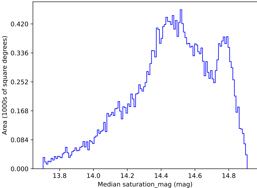
extra_ss_neo4_v3.4_10yrs All sky i band: Median saturation_mag
