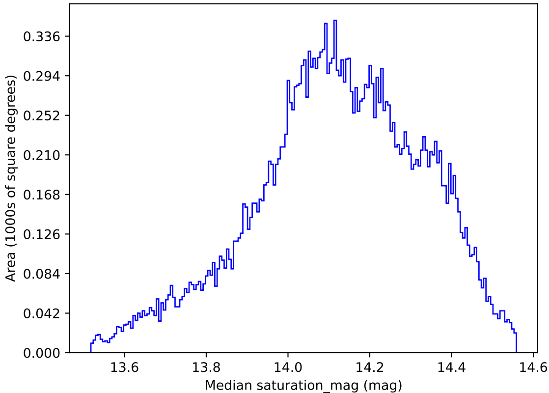
extra_ss_neo4_v3.4_10yrs All sky all bands: Median saturation_mag
