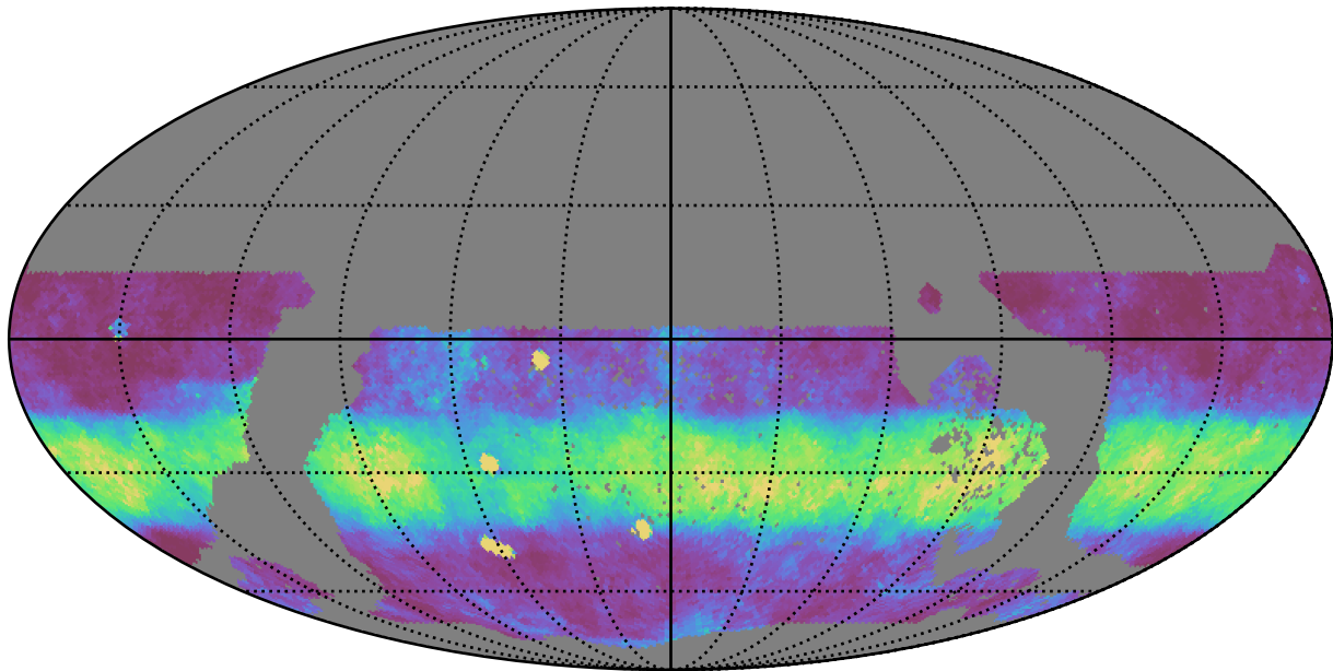
extra_ss_neo4_v3.4_10yrs WFD z band: Median normairmass
