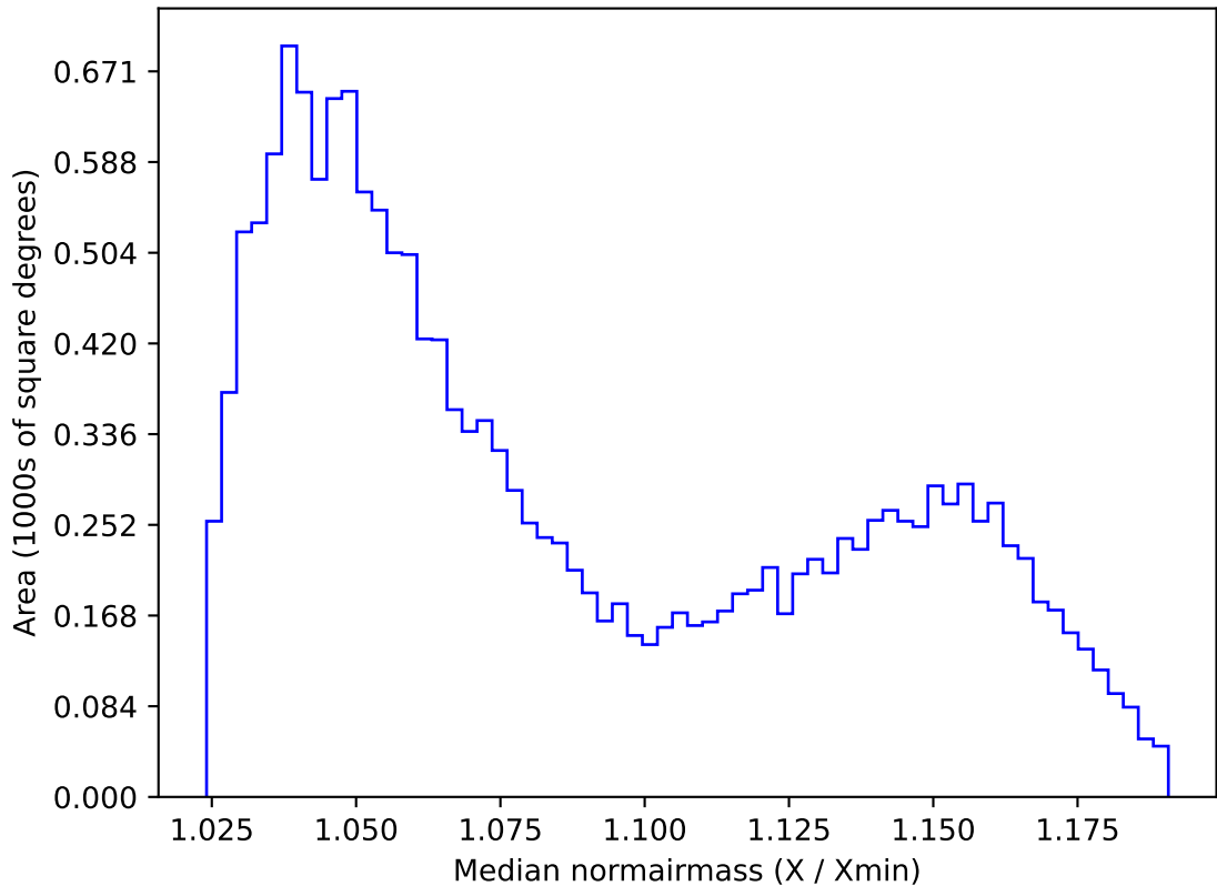
extra_ss_neo4_v3.4_10yrs WFD z band: Median normairmass
