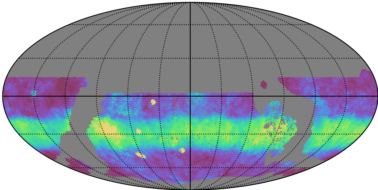
extra_ss_neo4_v3.4_10yrs WFD y band: Median normairmass
