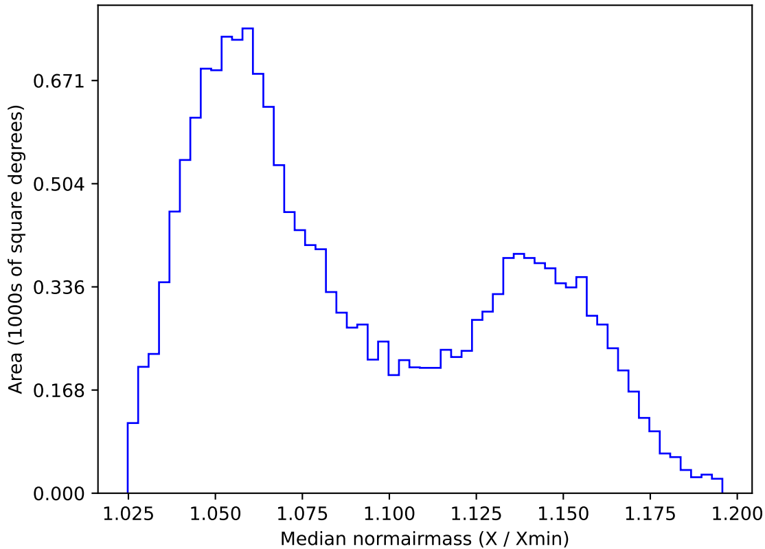
extra_ss_neo4_v3.4_10yrs WFD y band: Median normairmass
