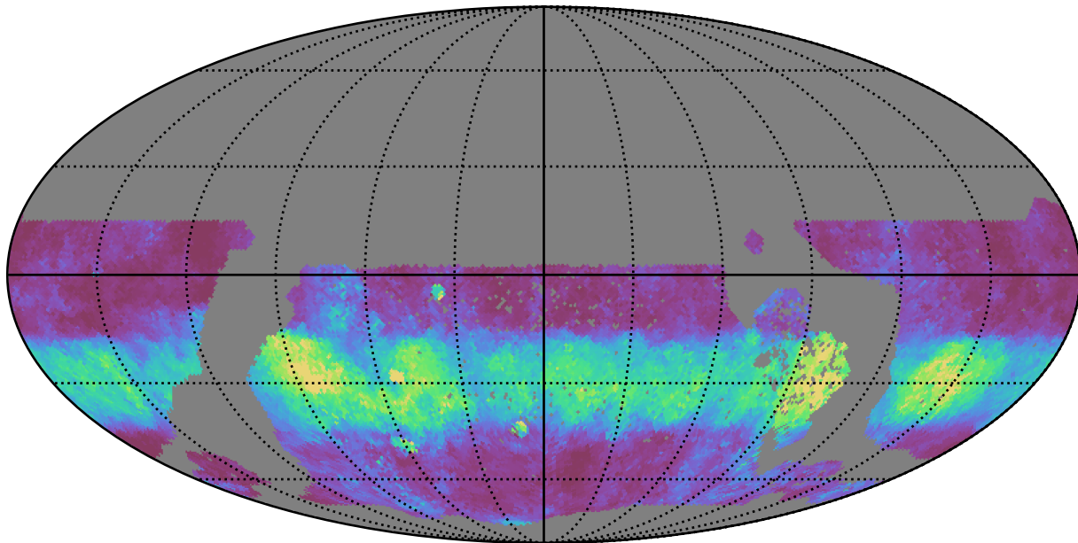
extra_ss_neo4_v3.4_10yrs WFD u band: Median normairmass
