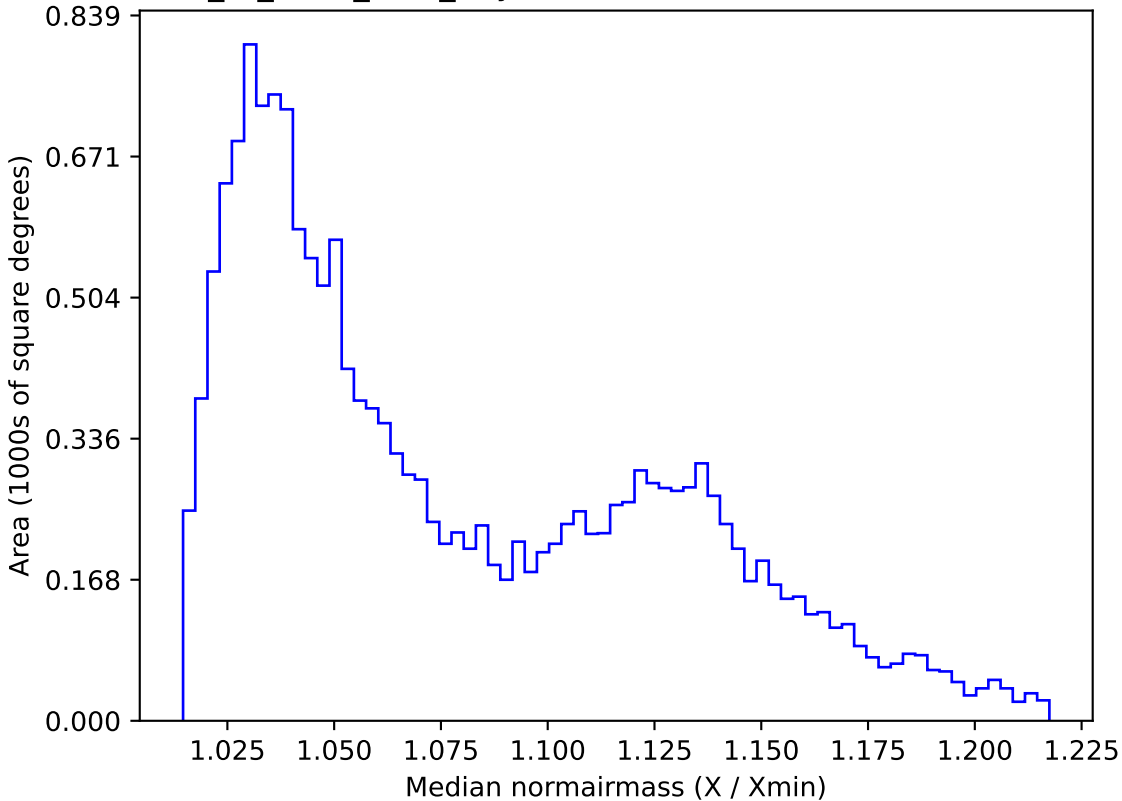
extra_ss_neo4_v3.4_10yrs WFD u band: Median normairmass
