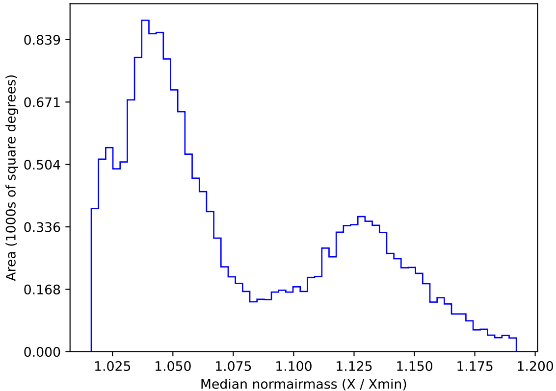
extra_ss_neo4_v3.4_10yrs WFD r band: Median normairmass
