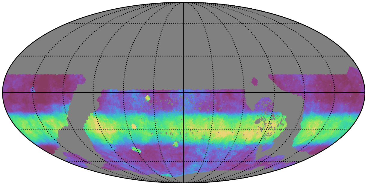
extra_ss_neo4_v3.4_10yrs WFD i band: Median normairmass
